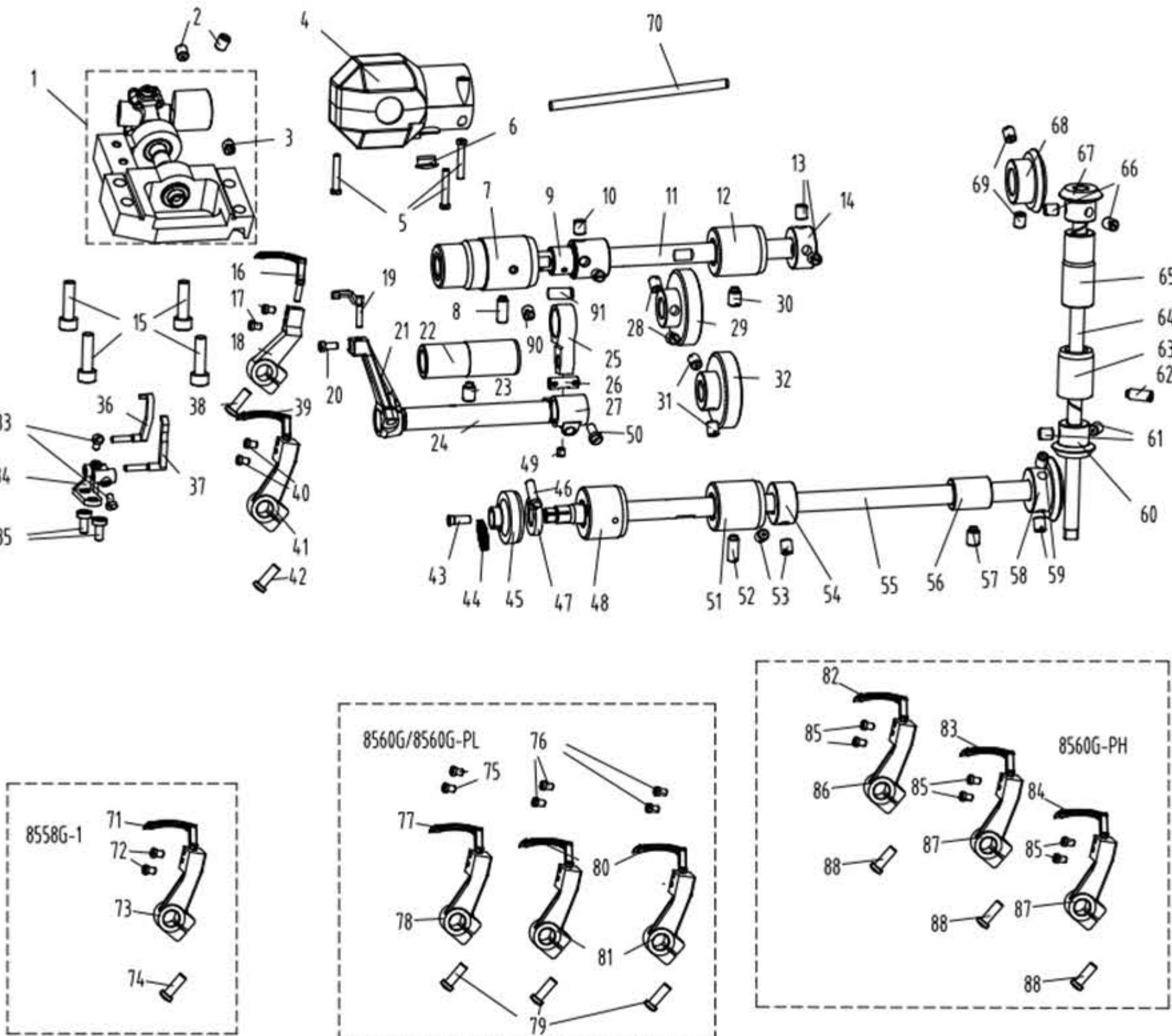
7. 弯针勾线分组件 Looper thread retainer components
